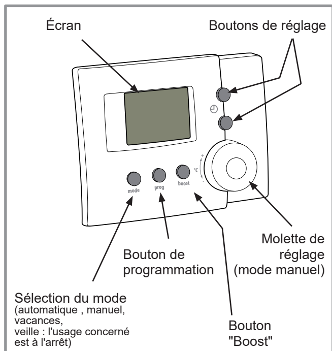
figure 5 - Sonde d'ambiance (option)
